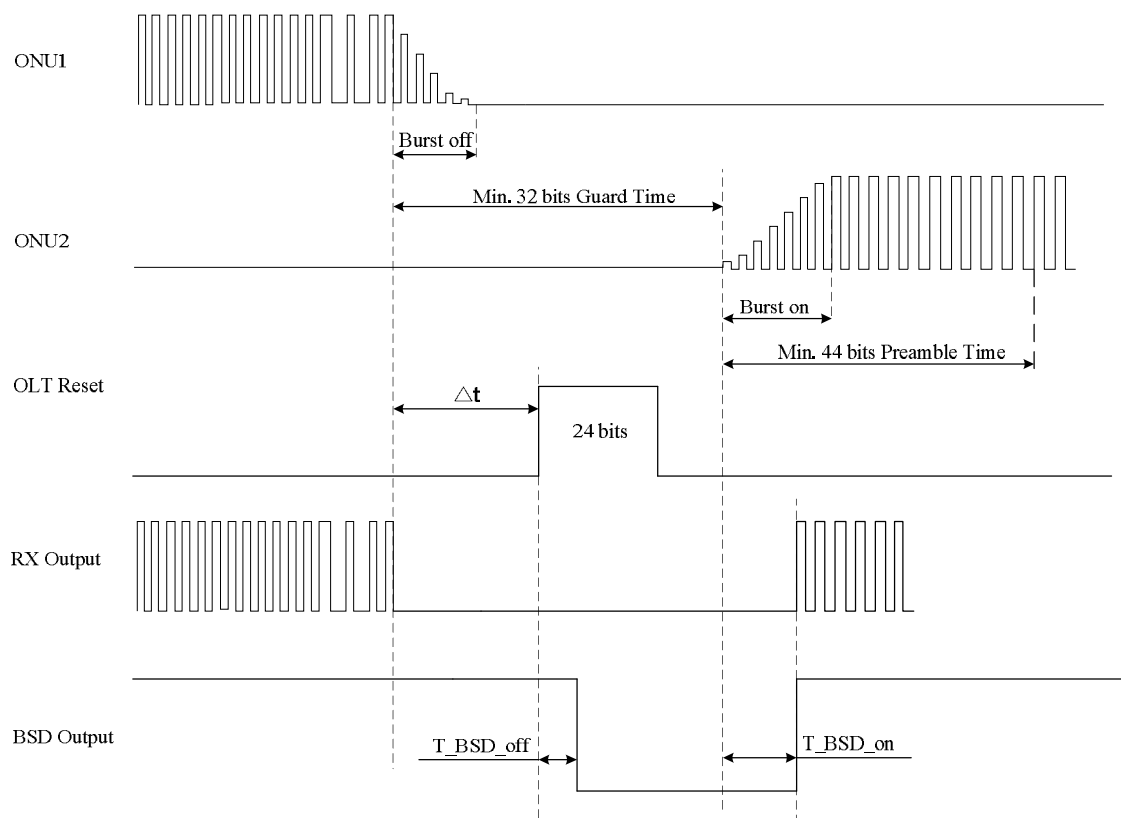
Figure 2 Reset Timin
